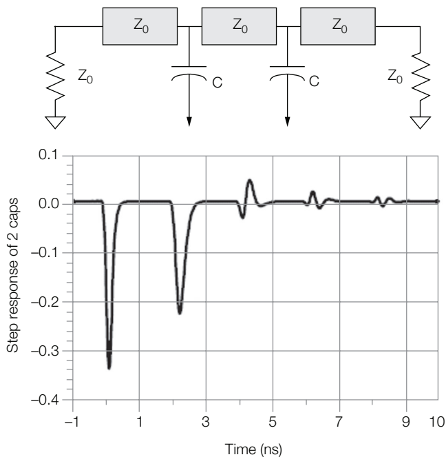
Figure 20. For two discrete identical discontinuities, response of the second discontinuity is somewhat masked by the first because not all energy reflected from the first discontinuity is available to be incident on the second.
