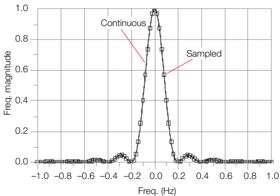
Figure 3a. Continuous function and discrete (sampled) function
