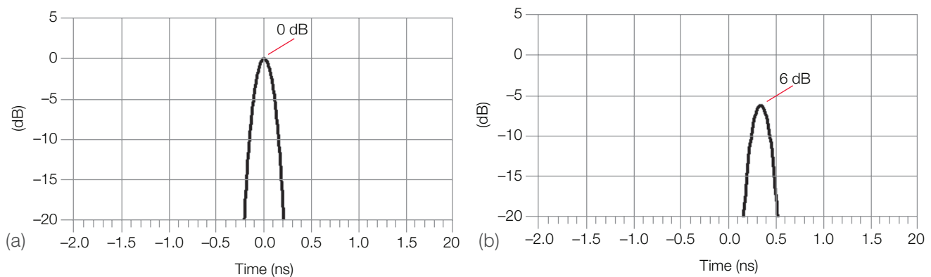
Figure 21. Impact of lossy network: (a) impulse response of a short circuit showing return loss of 0 dB, (b) time domain response of a 3 dB attenuator terminated with a short circuit, 6 dB loss represents the forward and return path loss through the attenuator.
