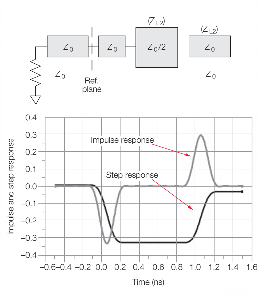
Figure 8. Showing a low-pass step and impulse responses of impedance changes (circuit shown above)
