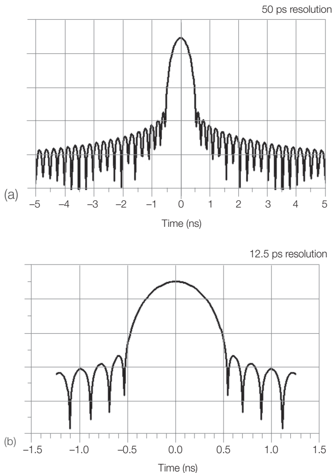
Figure 27. Range resolution: (a) a span of 10 ns results in a range solution of 50 ps, (b) reduce span to 2.5 ns and reduce resolution to 12.5 ps.
