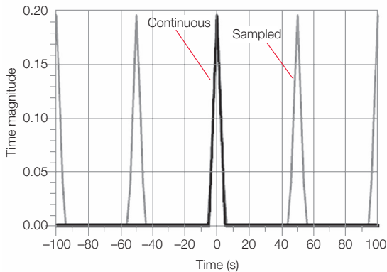
Figure 3b. Alias responses due to discrete sampling
