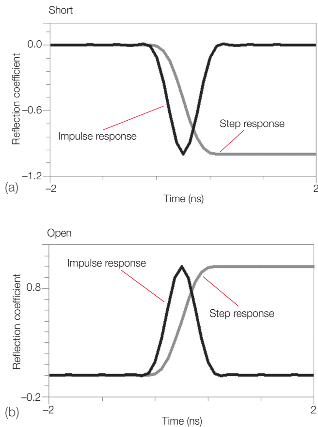
Figure 35. Low-pass responses of a short circuit (a) and an open circuit (b).
