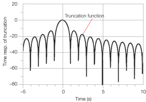
Figure 4b. Truncation causes ringing in time domain
