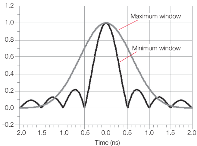
Figure 24. Comparing minimum window and maximum window
