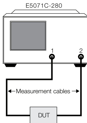
Figure 28. Equipment setup
