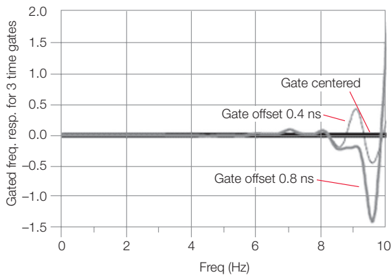
Figure 12c. Frequency response after gating
