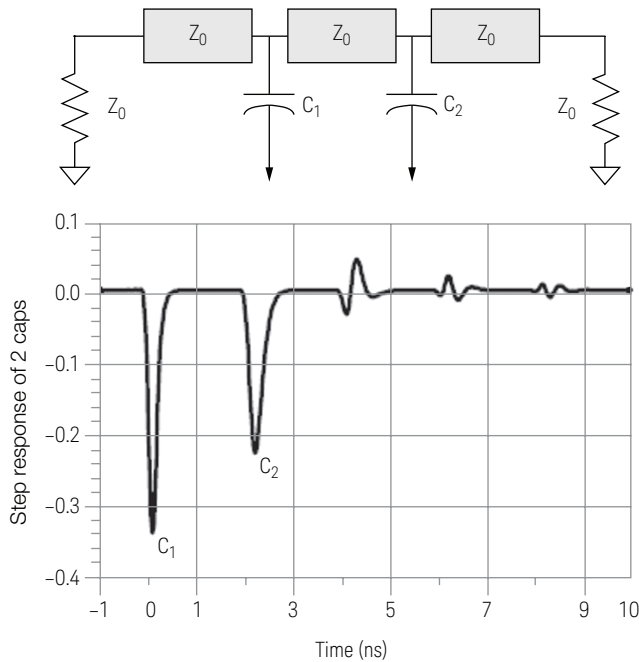
Figure 16. Time domain response of two capacitive discontinuities (circuit shown above)
